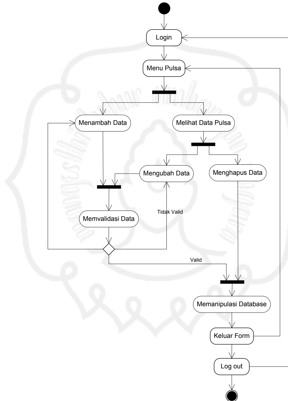
Gambar 3.5 Activity Diagram Mendata Pulsa
