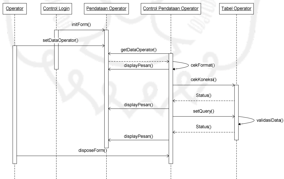
Gambar 3.14 Sequence Diagram Mendata Operator
