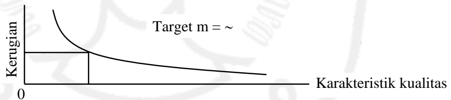
Gambar 2.11 Karakteristik larger the better
