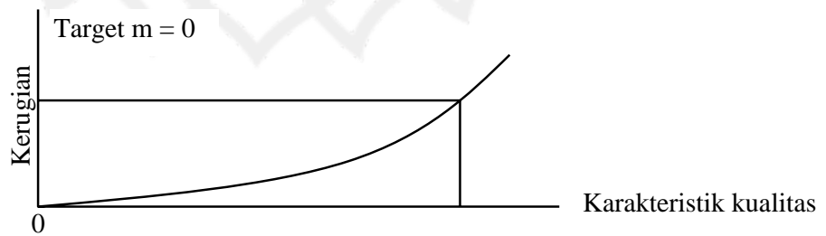
Gambar 2.10 Karakteristik smaller the better
