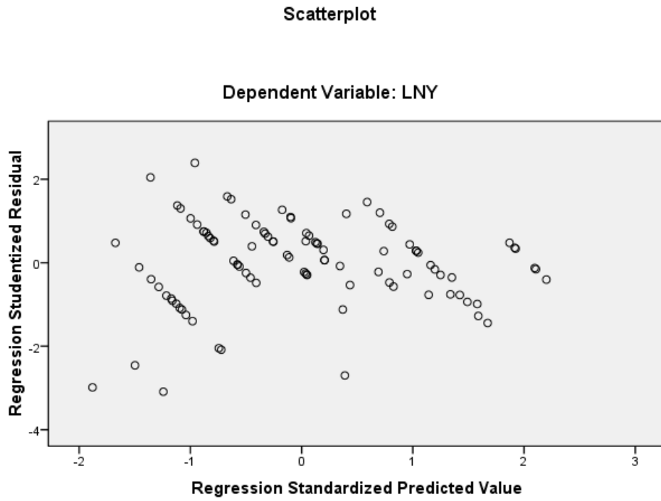
Gambar 6. Scatter Plot
