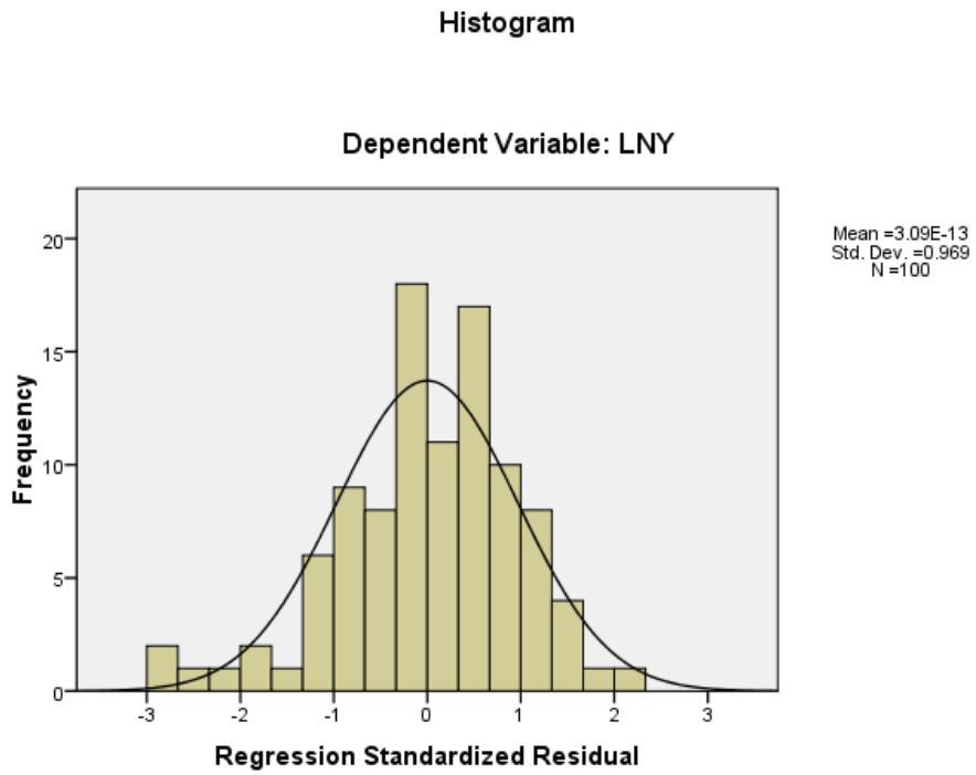
Gambar 4. Histogram
